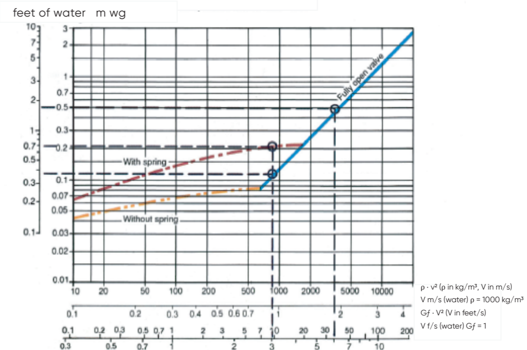
PRESSURE DROP - FLOW VELOCITY API 594, ANSI CLASS 150 - 300, HORIZONTAL PIPE (DIAGRAM 2)
