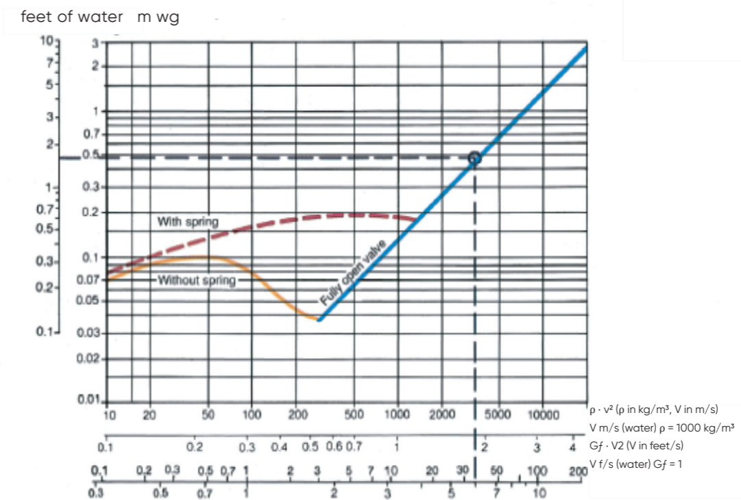
PRESSURE DROP - FLOW VELOCITY API 594, ANSI CLASS 150 - 300, VERTICAL PIPE (DIAGRAM 1)
